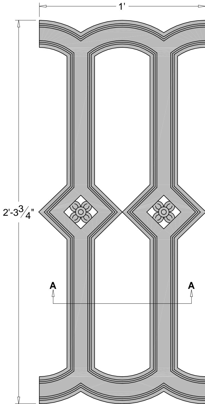
Front Elevation
