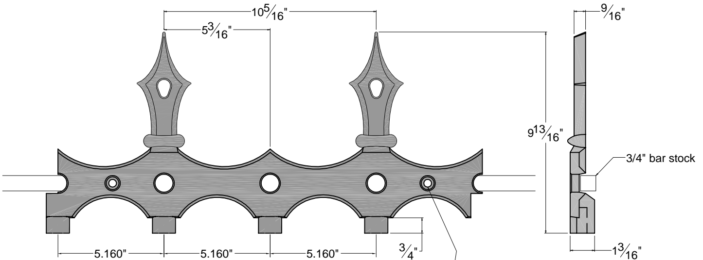
Side Elevation
