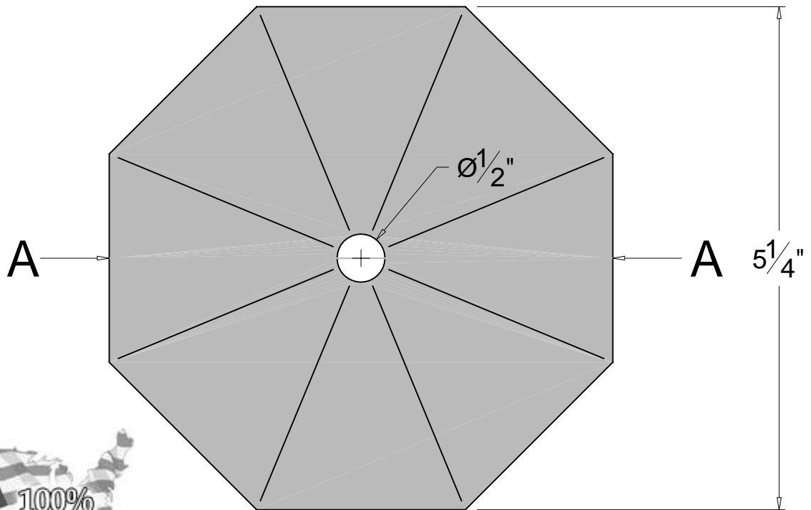
PLAN ELEVATION
