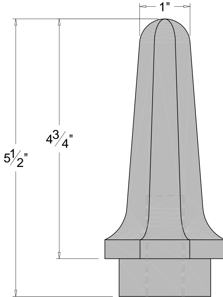
Front Elevation
