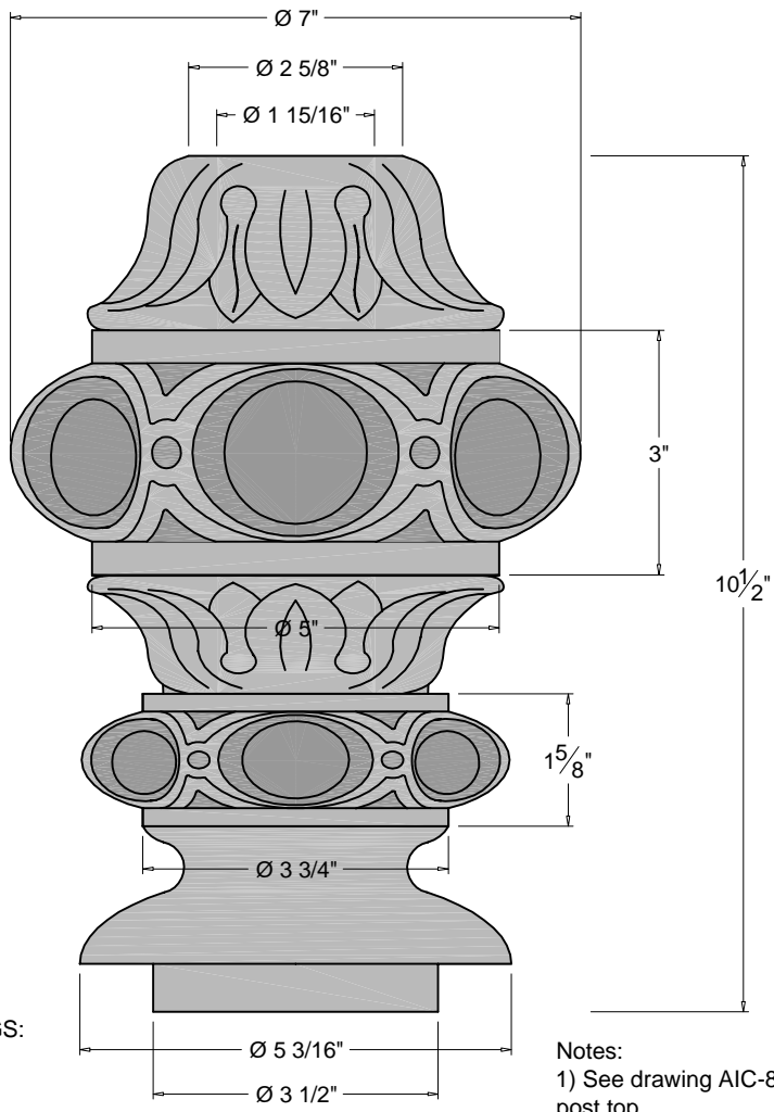
Front/Side Elevation
