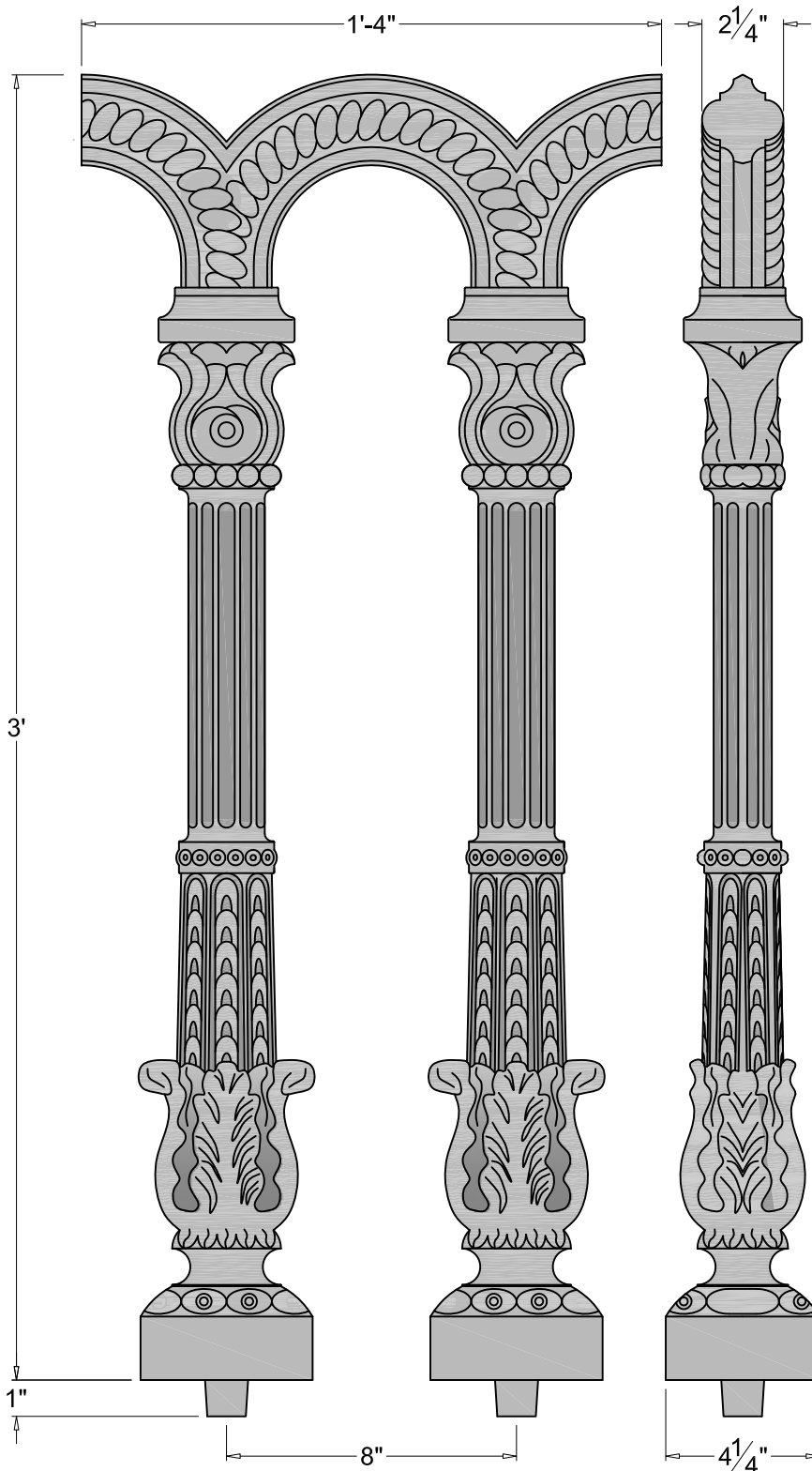
FRONT / REAR ELEVATION
