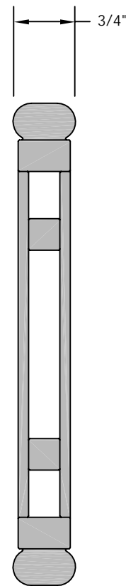
SECTION
