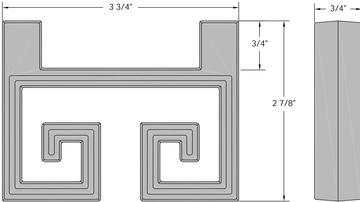
ELEVATION (FRONT & REAR SIMILAR)
