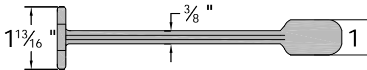
Side Elevation
