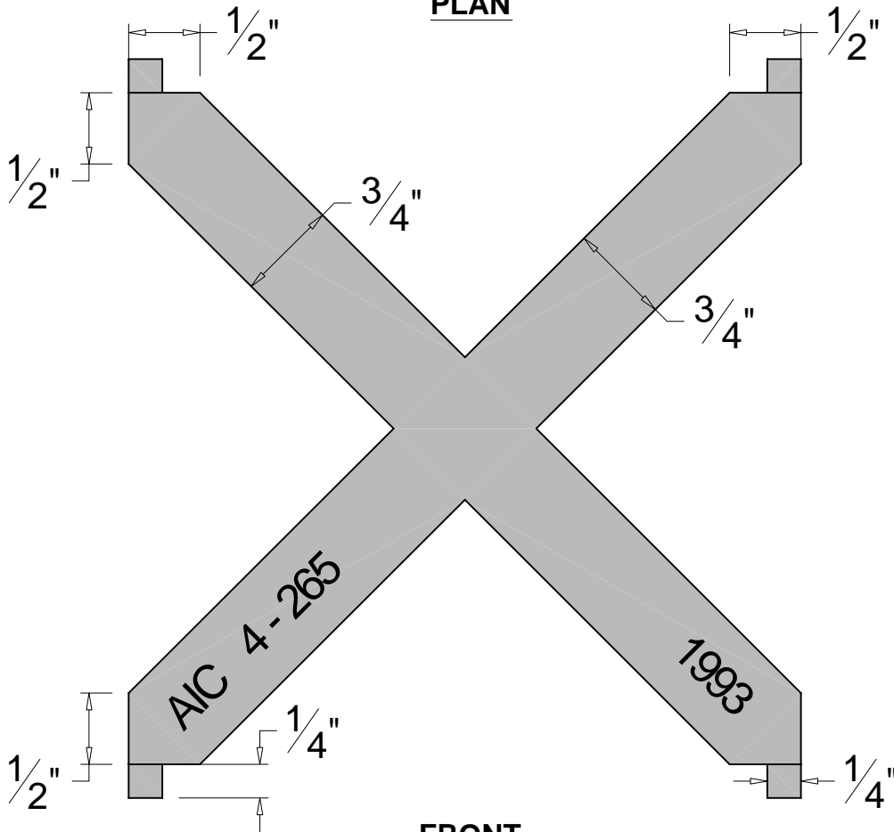
FRONT ELEVATION
