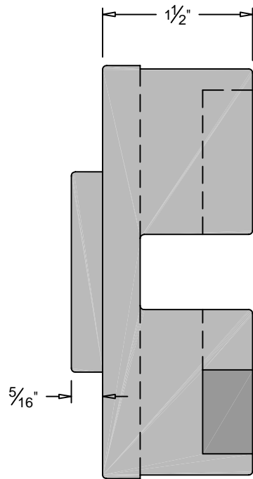
SIDE ELEVATION
