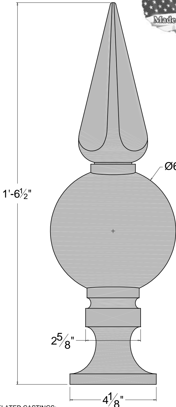
FRONT ELEVATION
