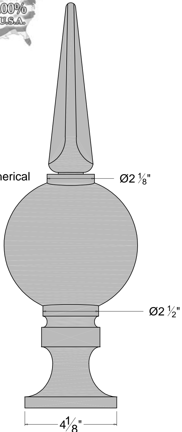
SIDE ELEVATION
