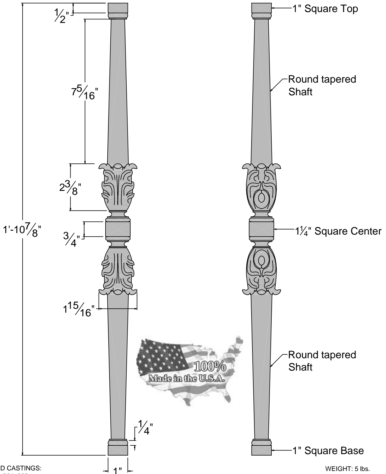
FRONT ELEVATION
