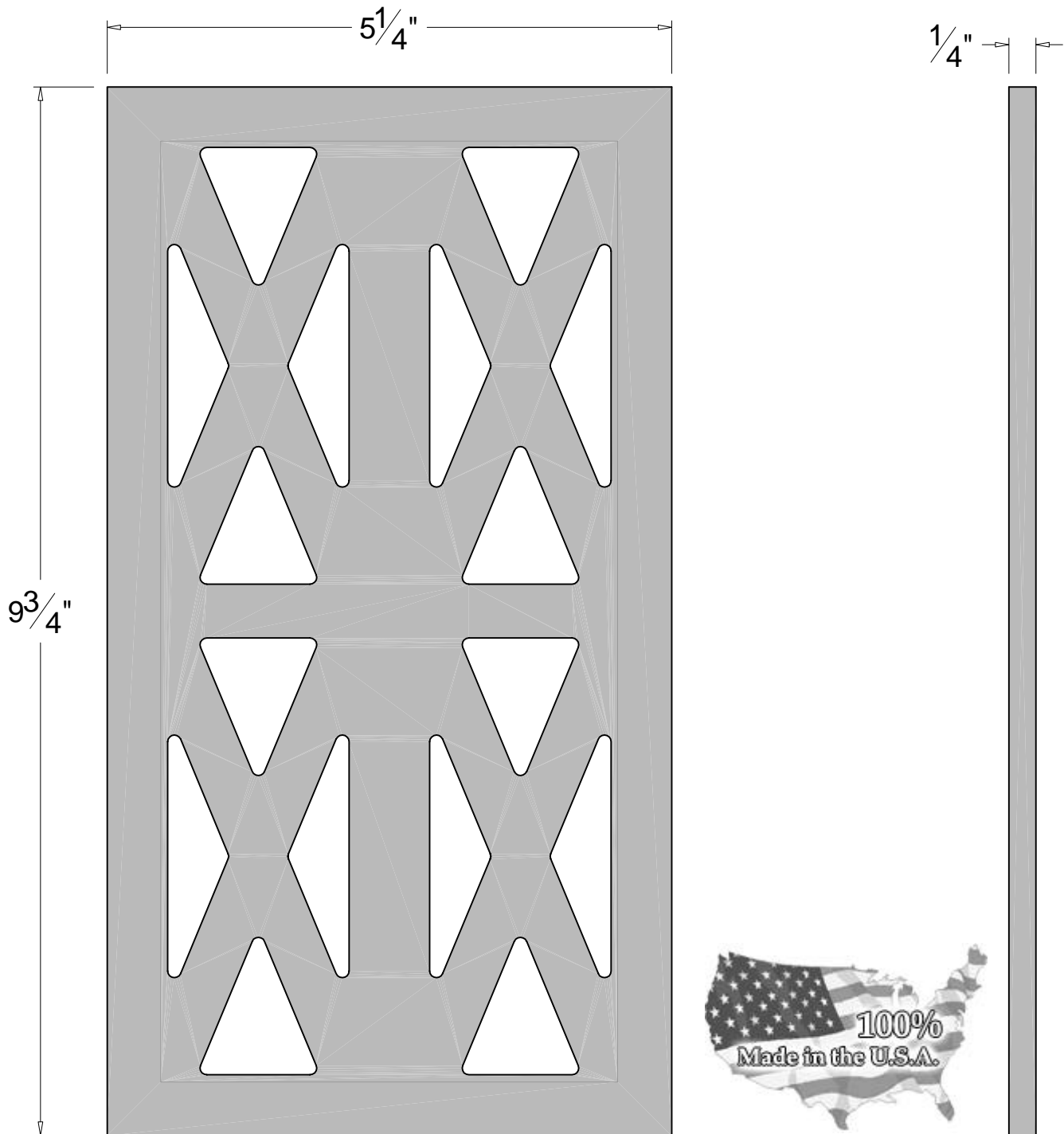
Front Elevation
