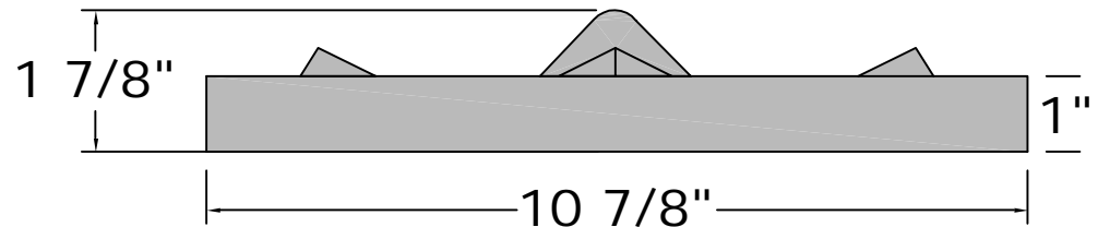
Side Elevation
