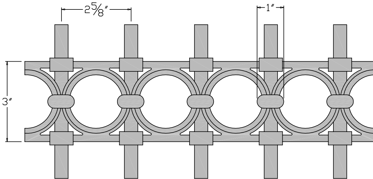
FRONT/BACK ELEVATION
