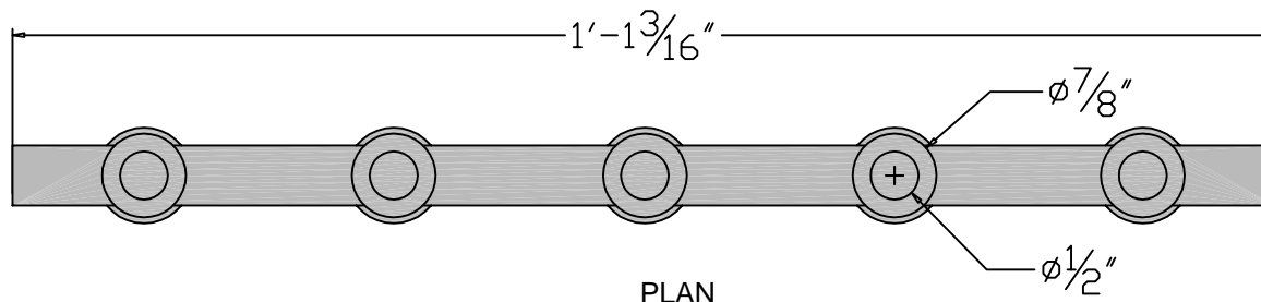
PLAN
