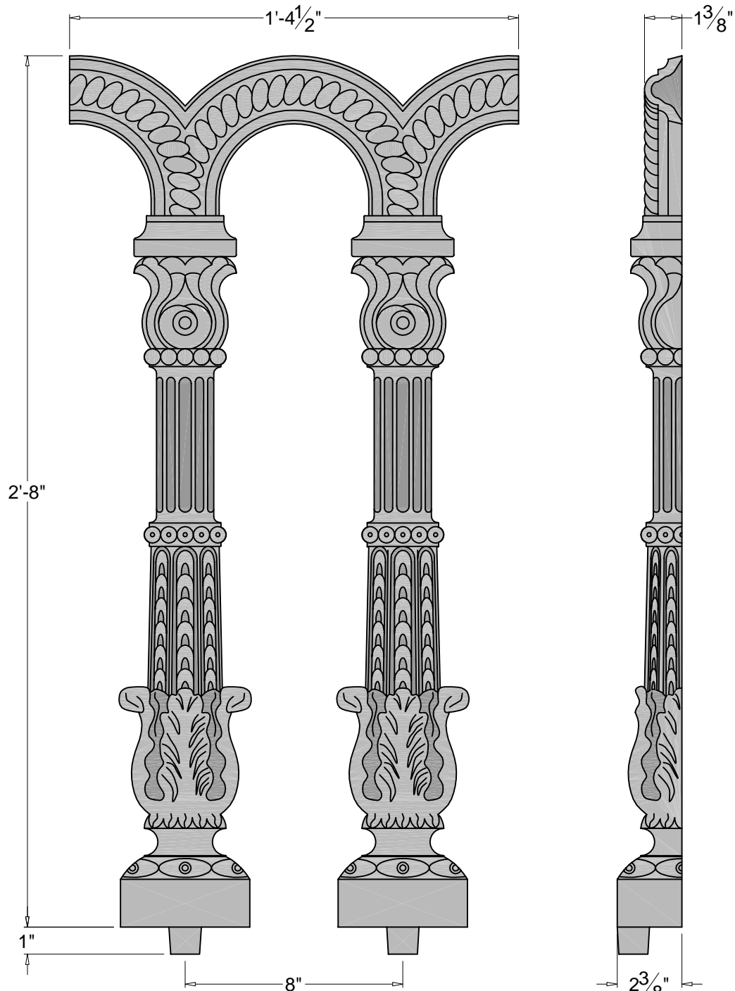
FRONT ELEVATION
