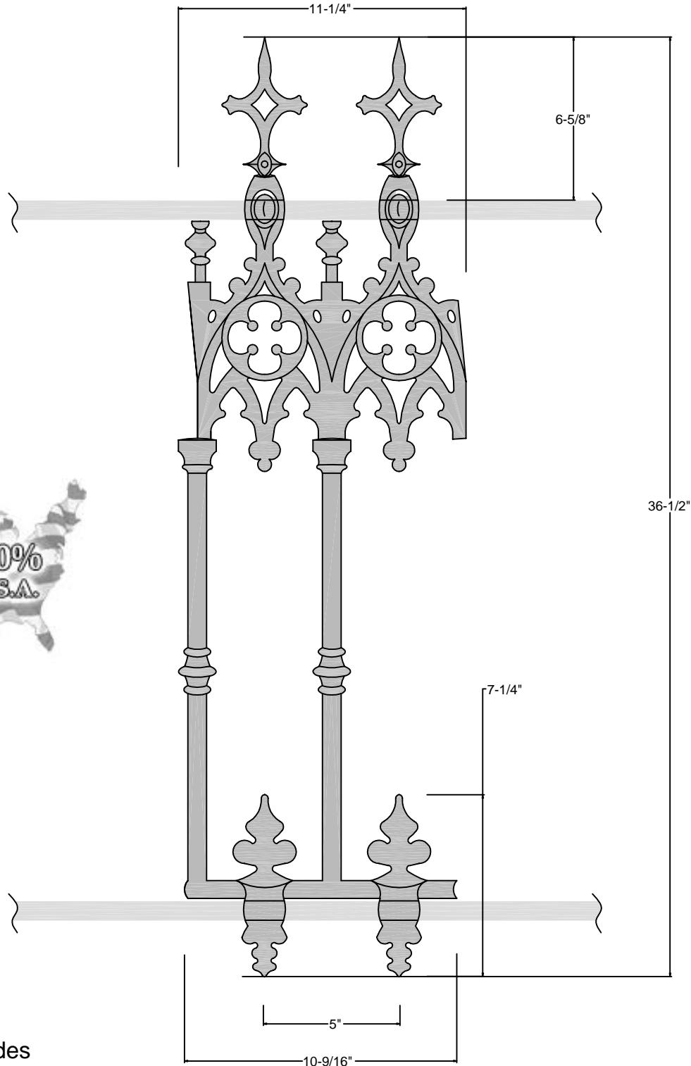
SIDE ELEVATION
