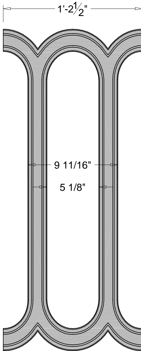
Front Elevation
