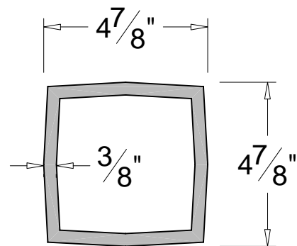
Cross Section at A
