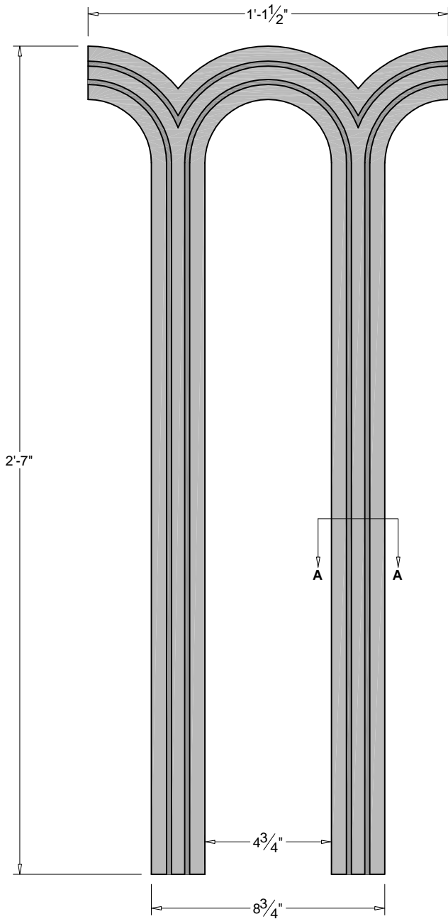
Front Elevation
