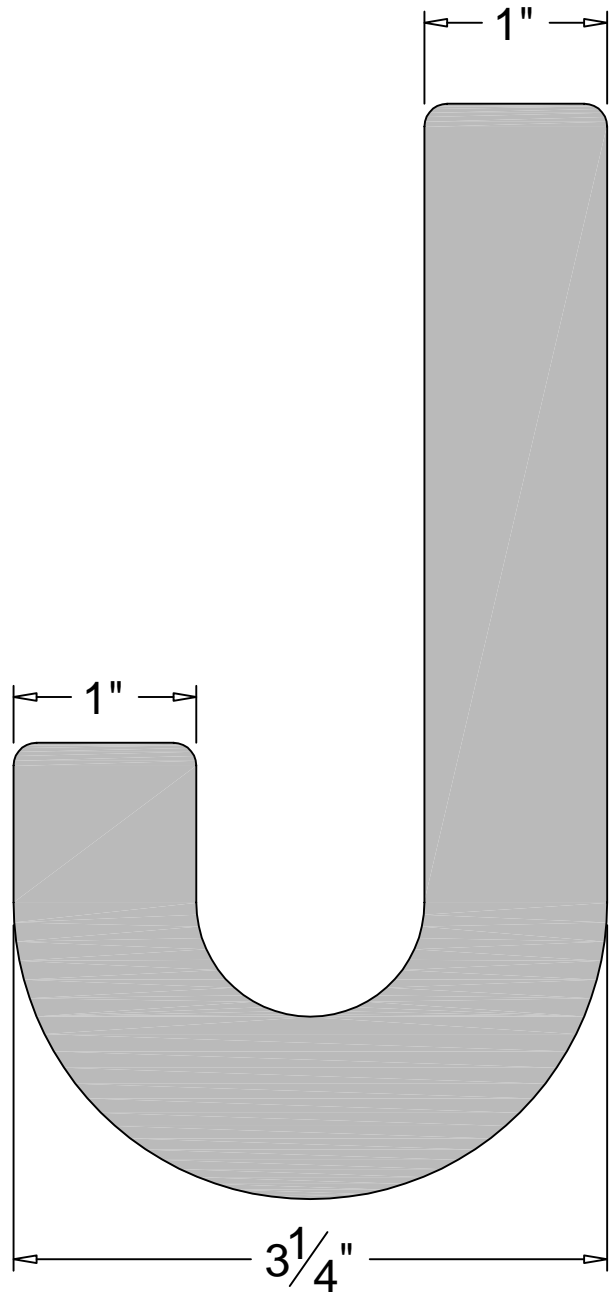
FRONT EVELVATION
