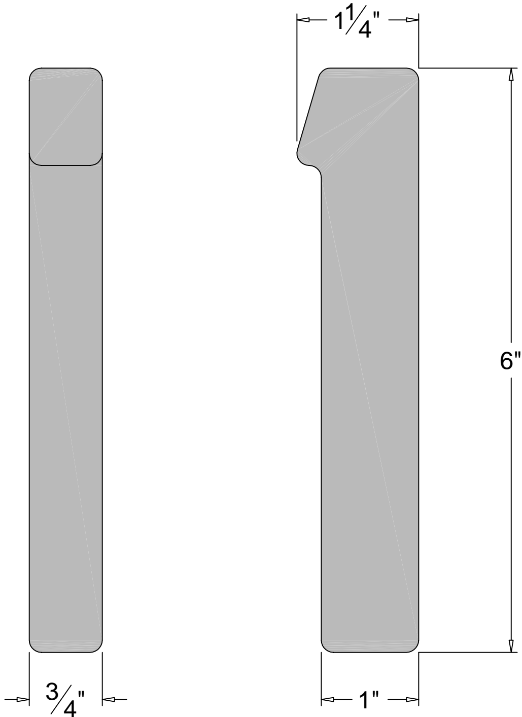
FRONT EVELVATION
