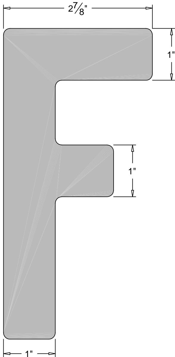
FRONT ELEVATION
