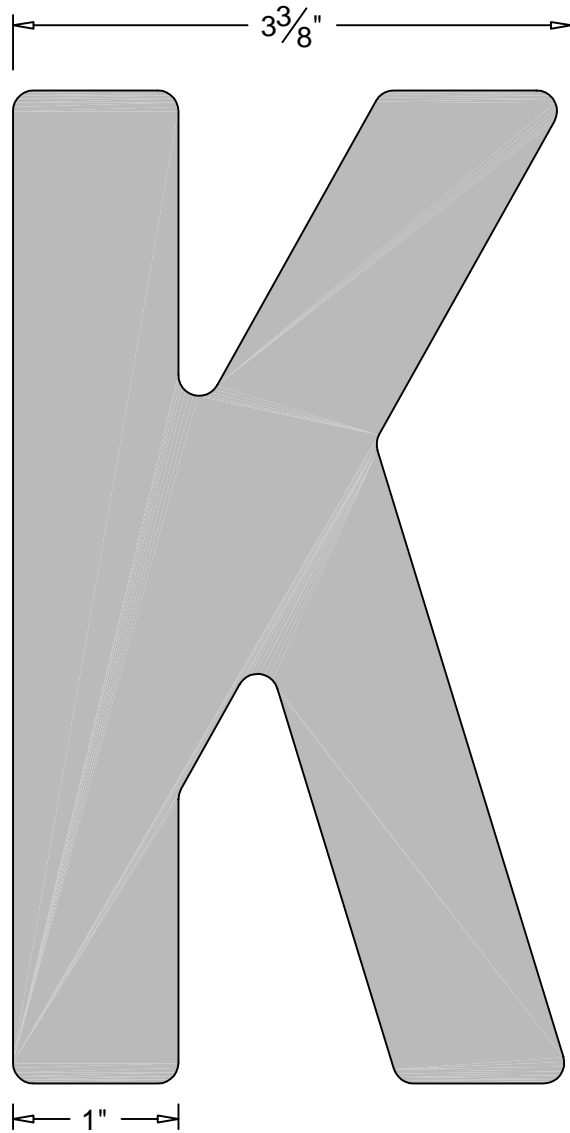
FRONT ELEVATION
