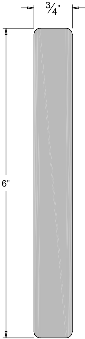
SIDE ELEVATION
