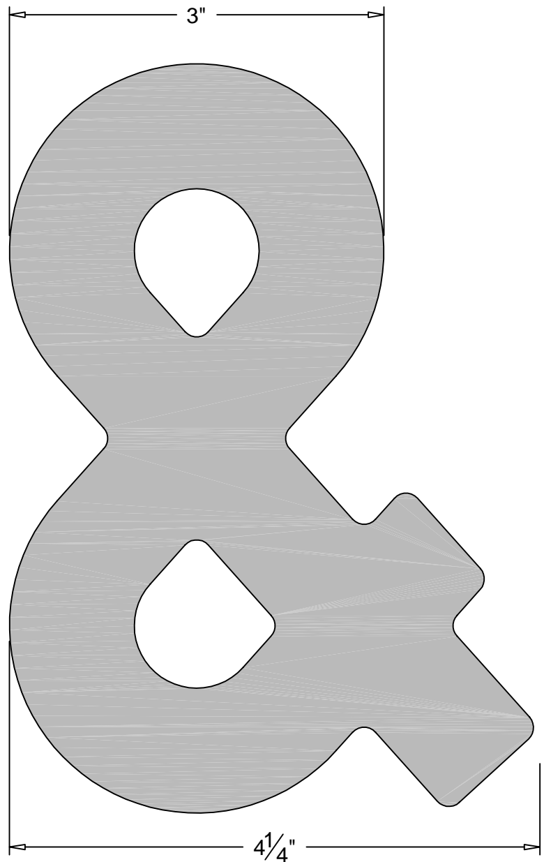
FRONT ELEVATION
