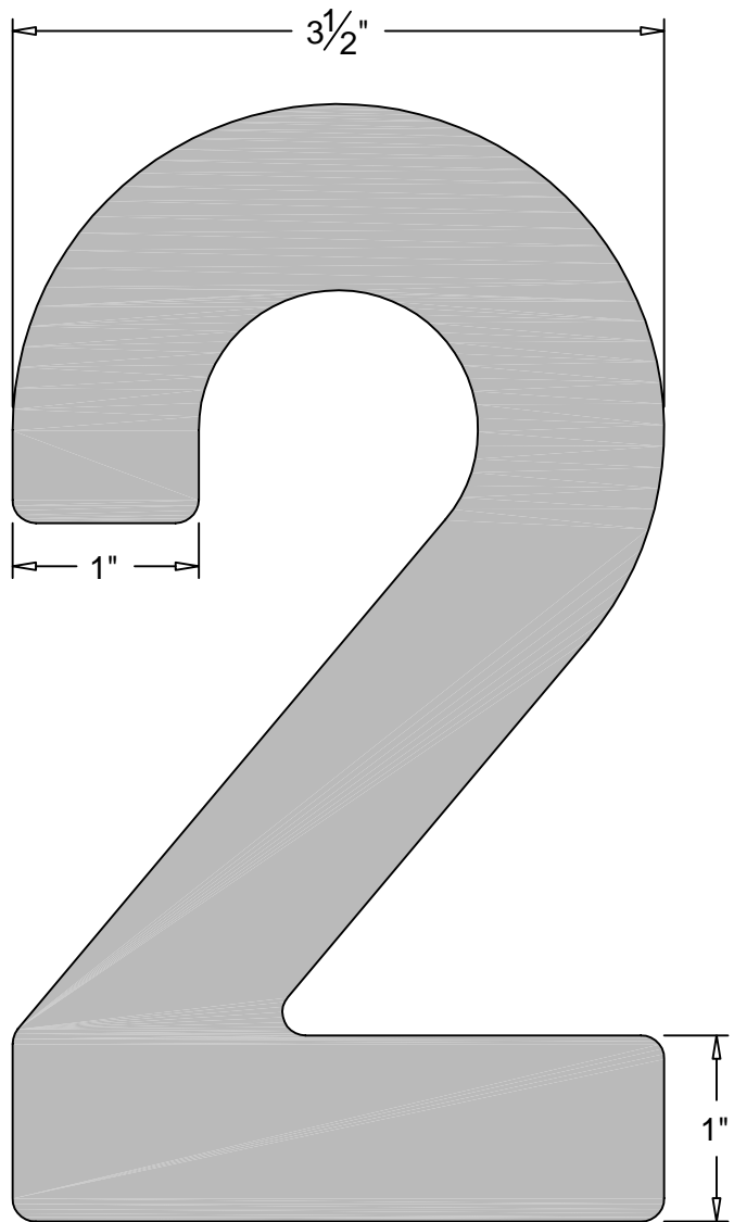
FRONT ELEVATION
