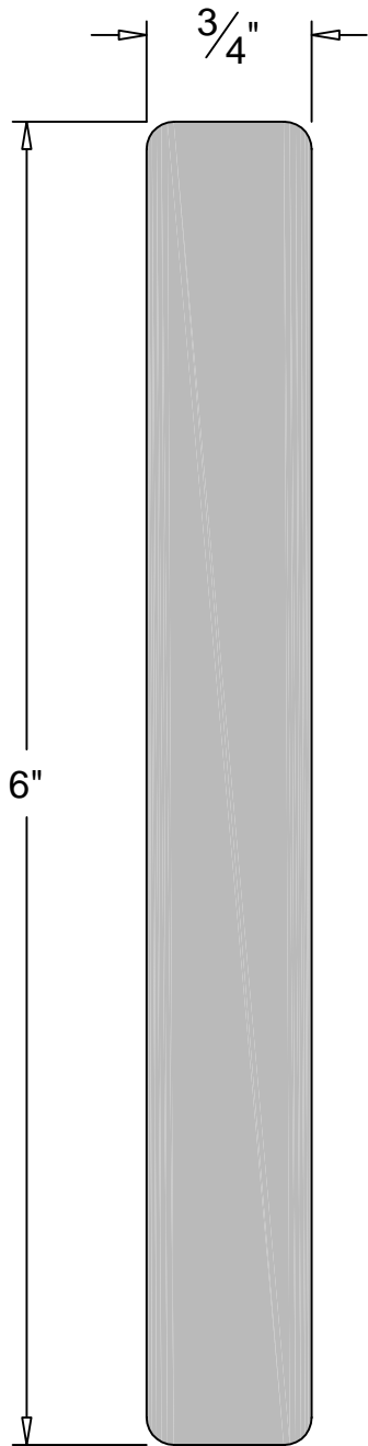
SIDE ELEVATION
