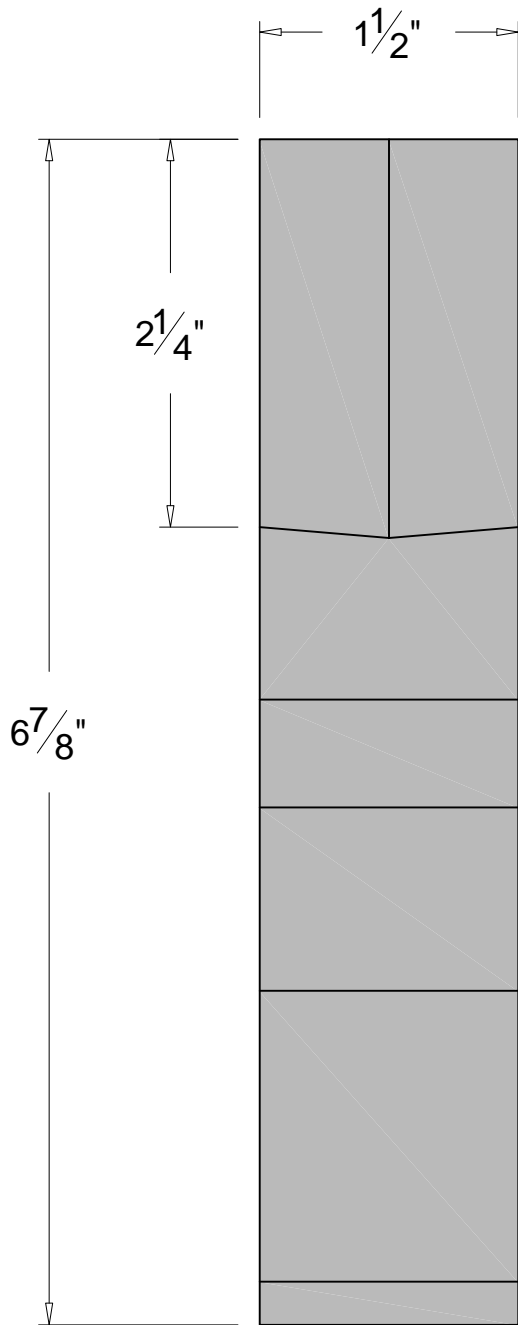
Front Elevation
