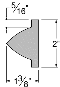
END ELEVATION & Typical Section
