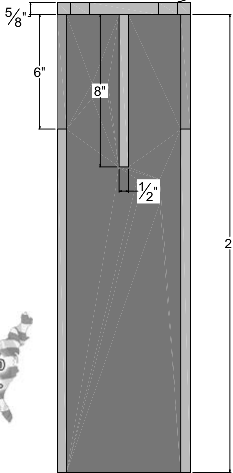
Back Elevation
