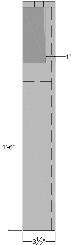
Side Elevation
