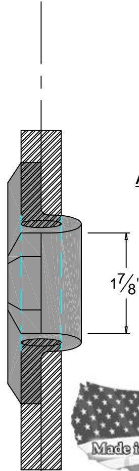
SIDE ELEVATION
