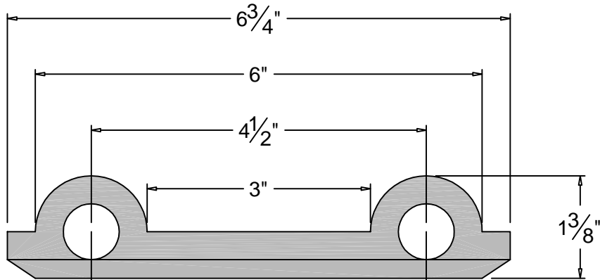
TOP/PLAN ELEVATION
