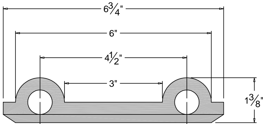
TOP/PLAN ELEVATION
