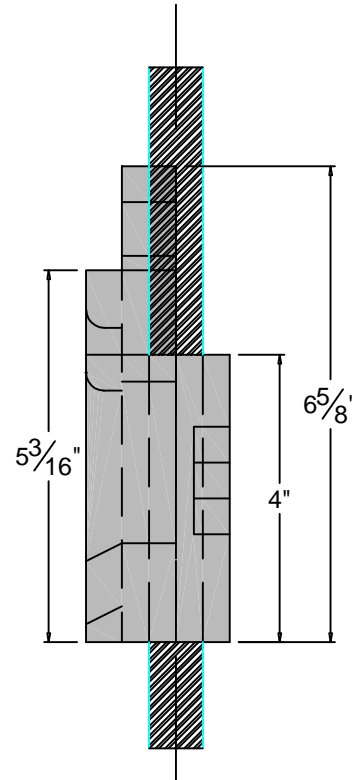
SIDE ELEVATION
