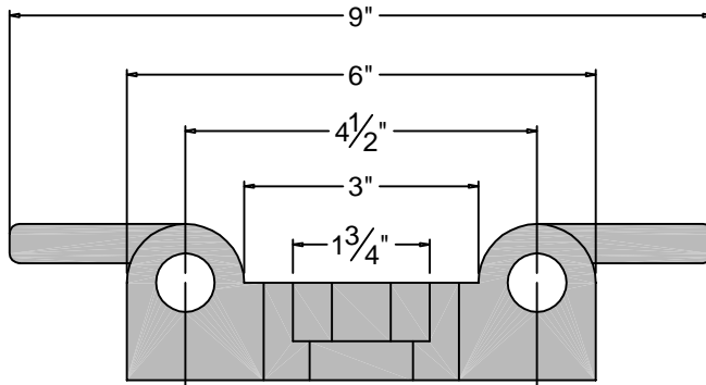
TOP/PLAN ELEVATION
