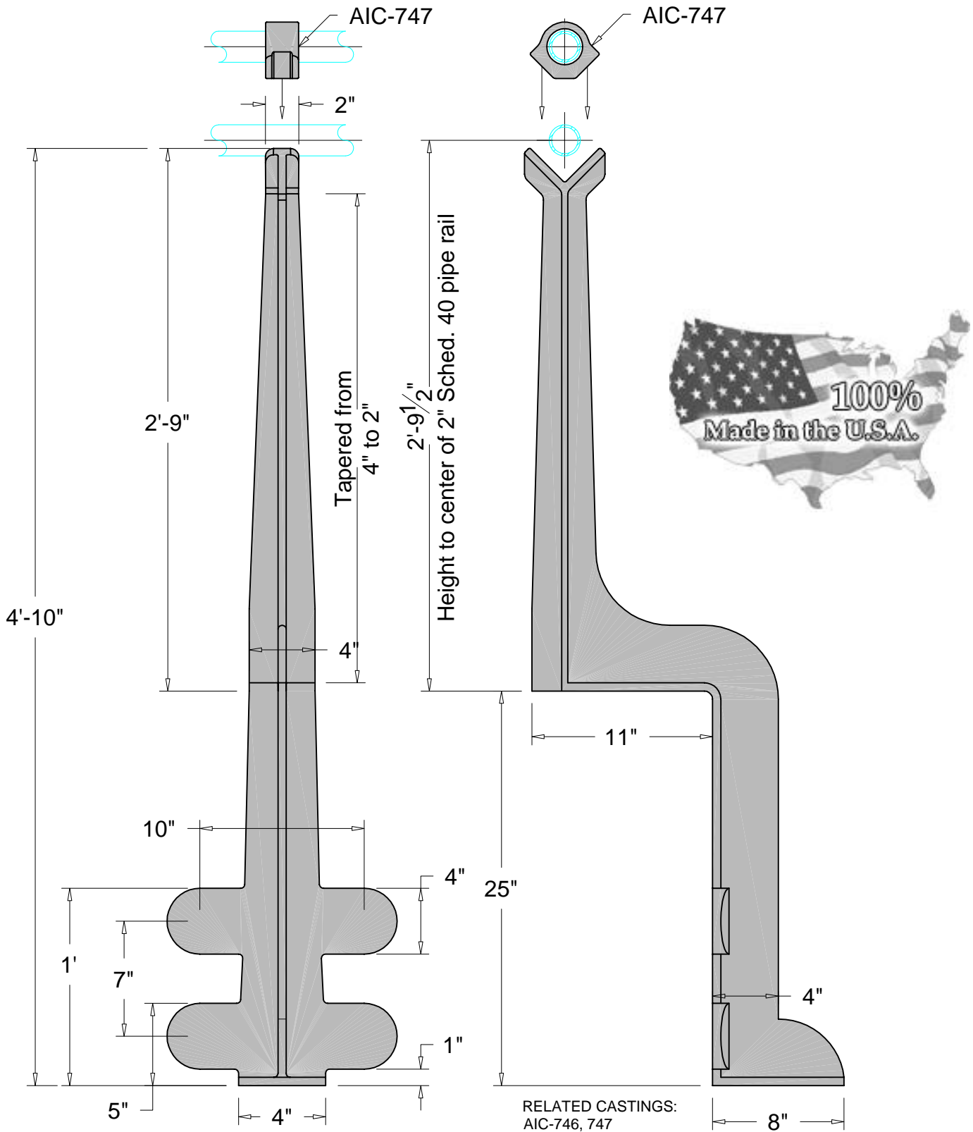
Front Elevation
