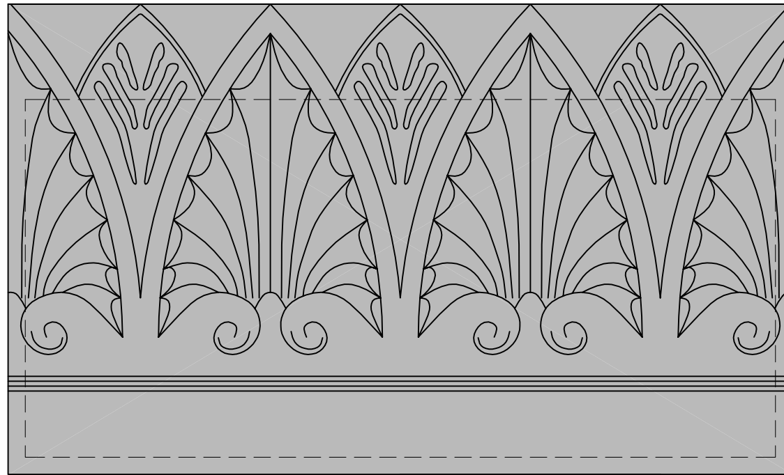
Front Elevation
