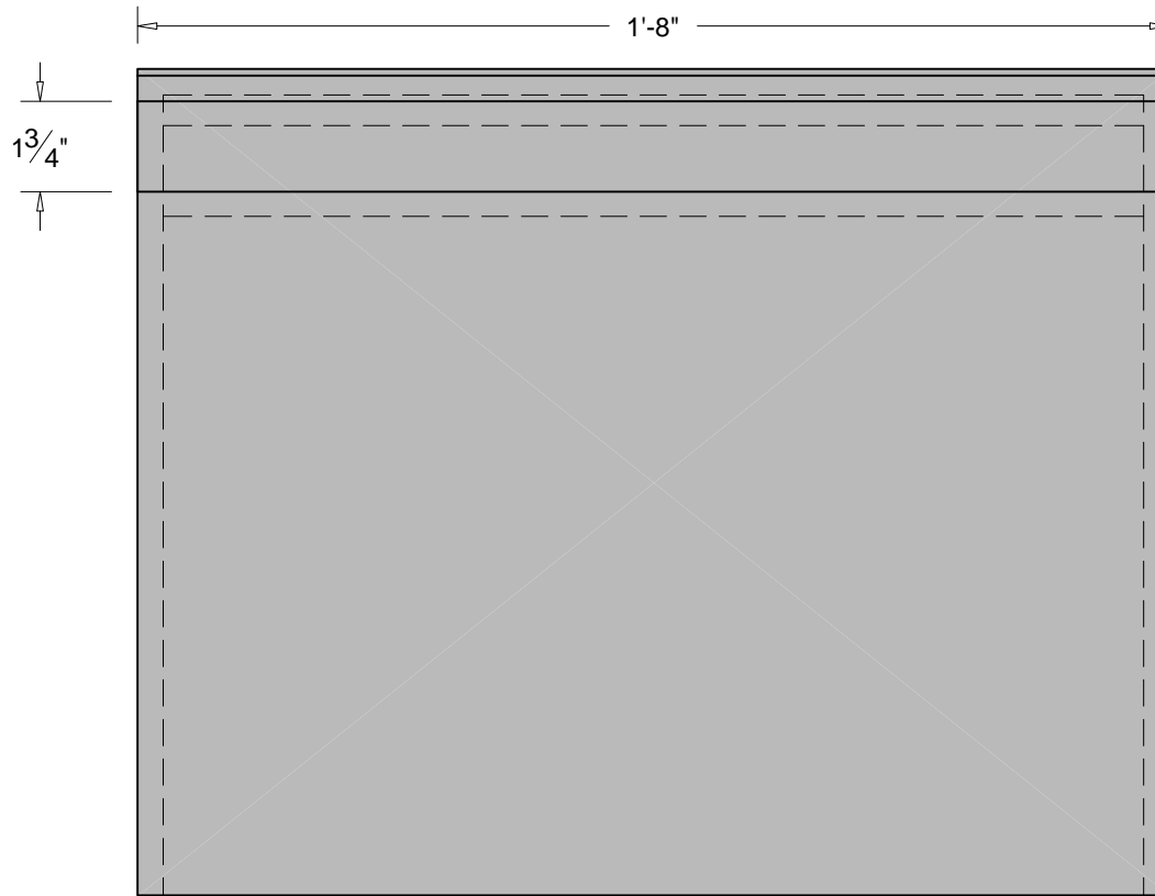
Front Elevation
