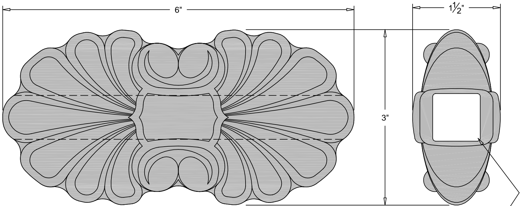
PLAN
