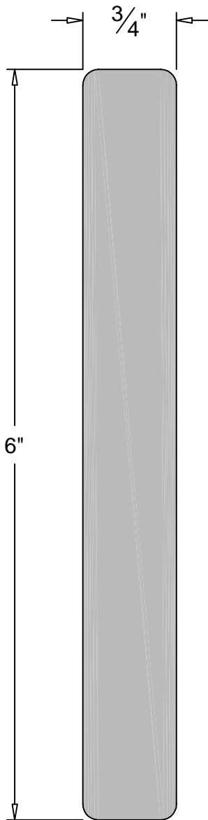
SIDE ELEVATION
