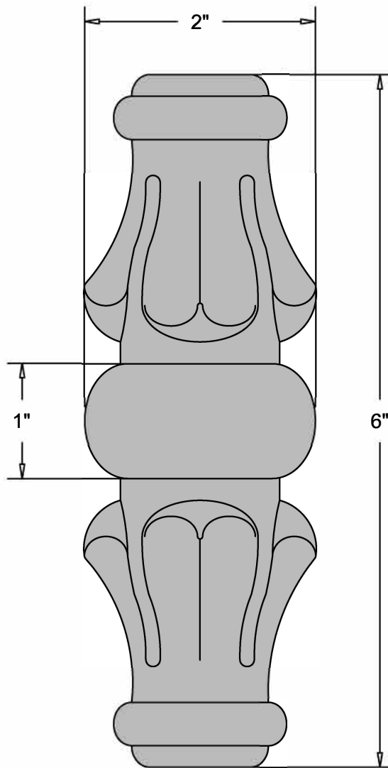
FRONT ELEVATION
