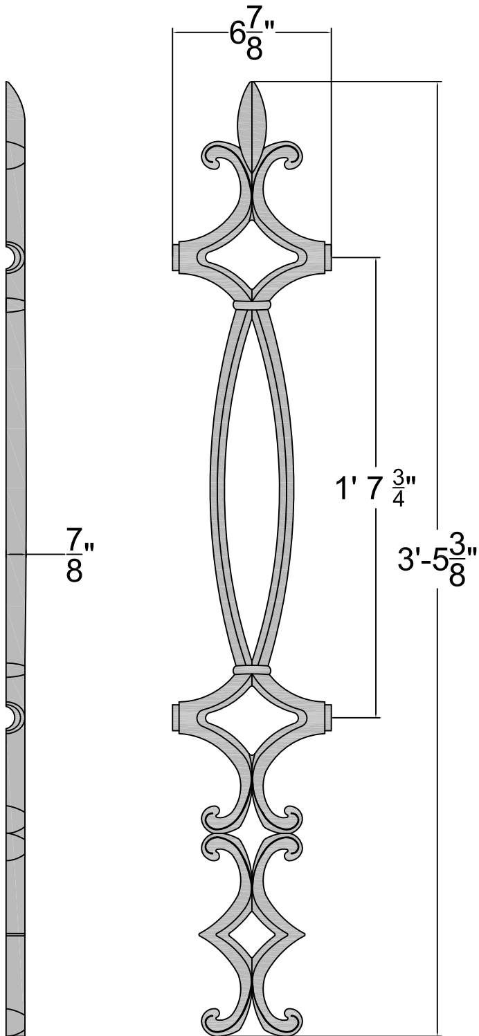
Front Elevation
